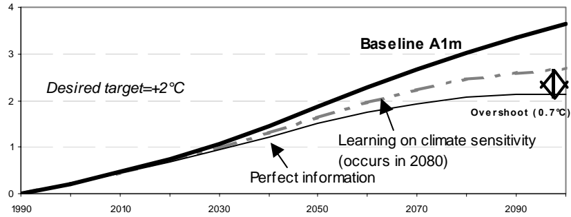
Figure 4 Comparing the cost of misestimating belief on climate change damages and climate dynamics
