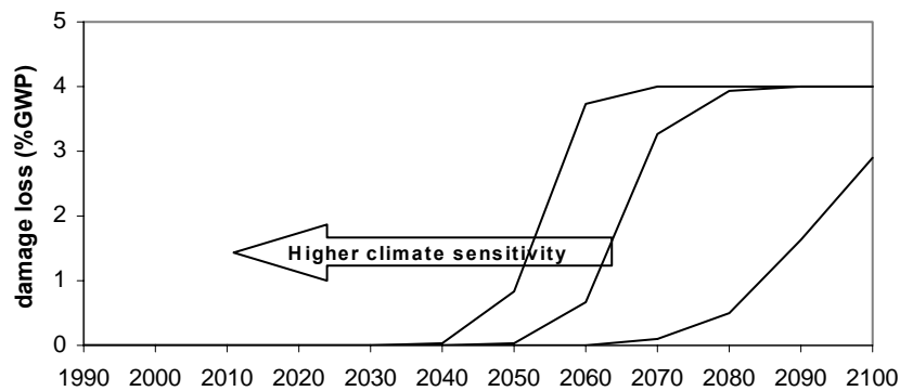
Figure 7 Depending on the value of climate sensitivity, in the case of singularities around a +2°C warming threshold, abrupt shifts (in the baseline case) occur sooner as climate sensitivity is higher
