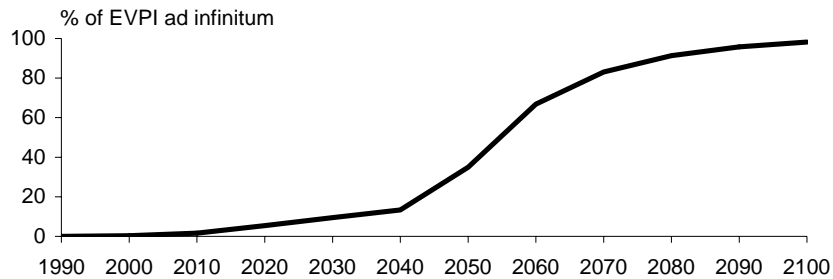
Figure 2 Expected Value of Perfect Information with respect to the date of resolution of uncertainty on climate sensitivity. Information value raises brutally after 2040, that means there is a significant interest in revealing this value before this date [17].
