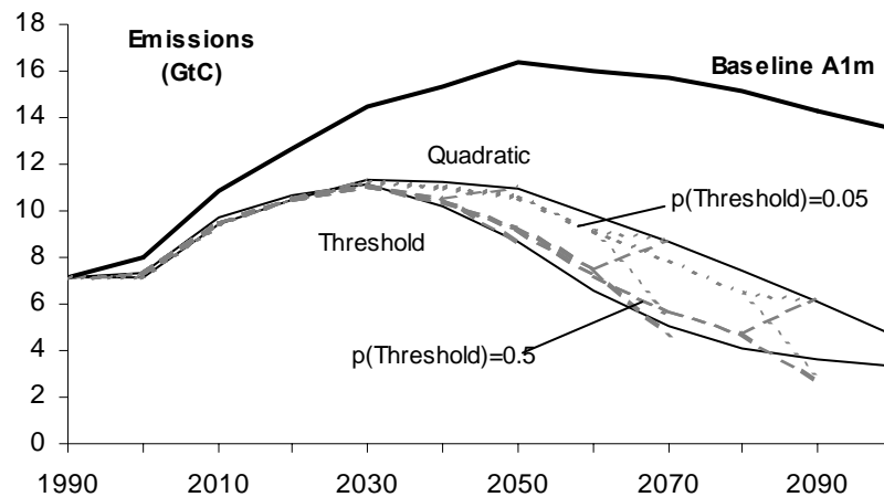
Figure 10 Emissions paths for different subjective probabilities of the threshold function with learning Threshold function probability : 0% for the upper thin black line; 5% for the dotted grey line, 50% for the dashed grey line; 100% for the lower thin black line. Learning occurs in 2040, 2060 and 2080
