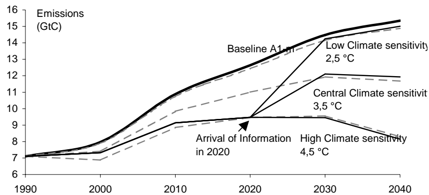
Figure 1 Hedging strategies for a given +2°C temperature ceiling : with perfect information (grey broken line) and with uncertainties (black solid line)
