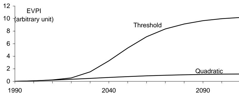
Figure 9 Expected Value of Perfect Information on climate sensitivity for quadratic and threshold damage functions
