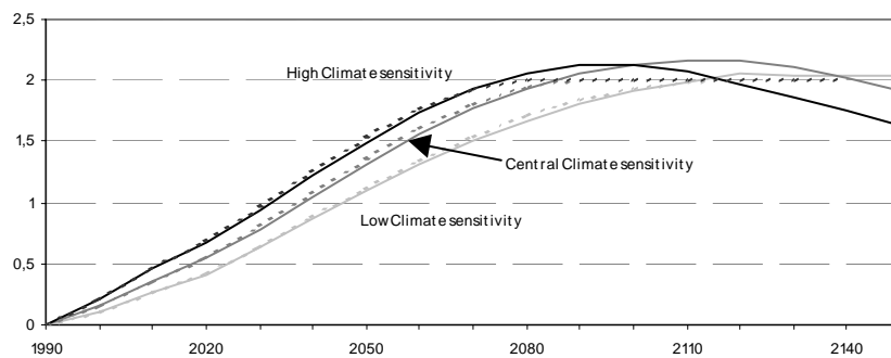
Figure 3 Global mean temperature increase for 3 climate sensitivities In a cost-benefit analysis with Pure Preference for Current Climate Regime based on a desired 2°C target (solid line) and in a cost-efficiency analysis with a 2°C target (broken line).
